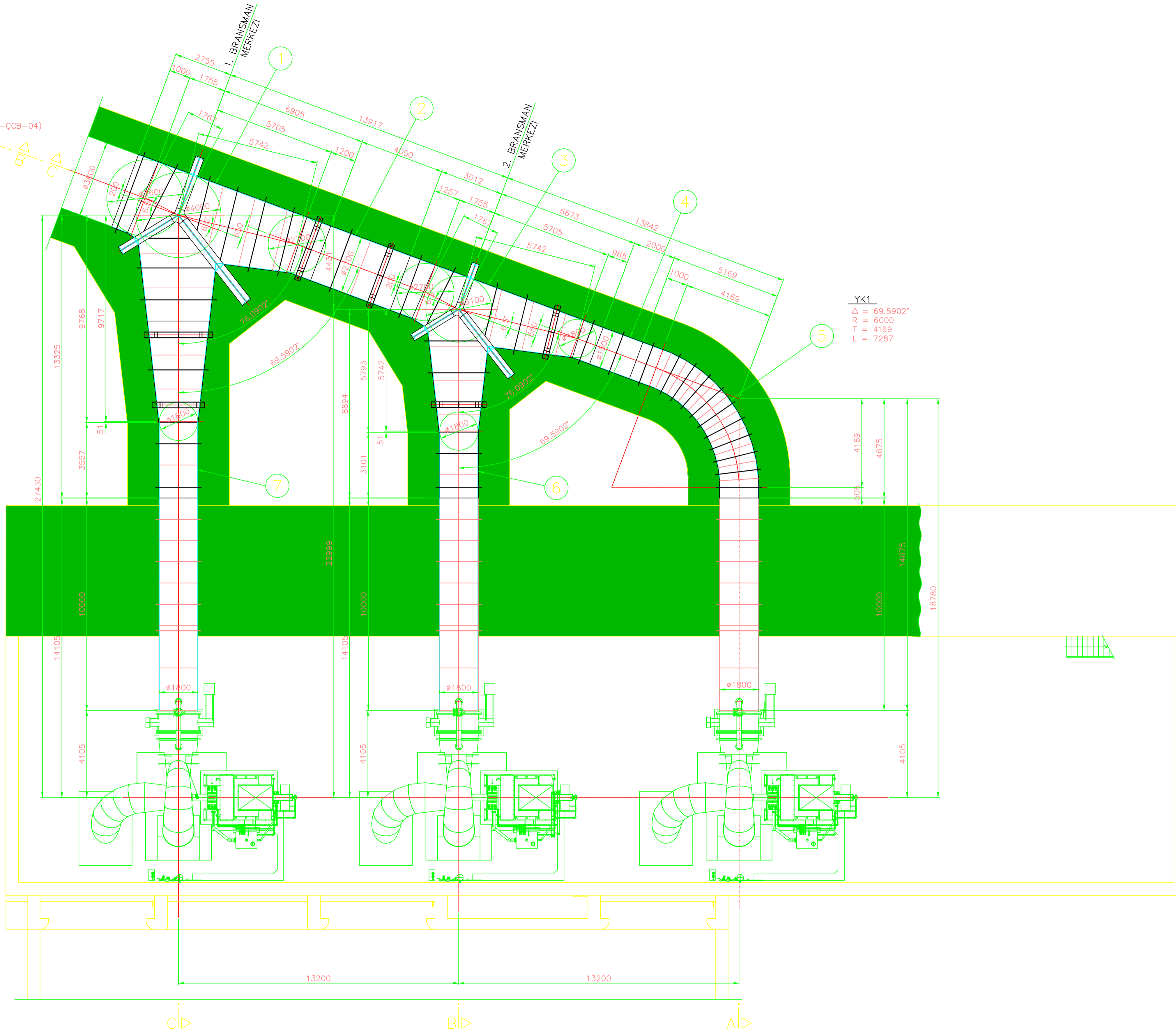
BRANSMAN BOLGESI PLANI 1/100
